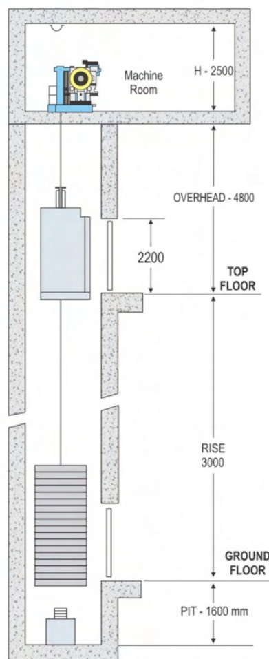
HOISTWAY ELEVATION DRAWING
