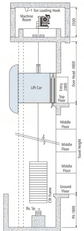
Hoistway Elevation Plan
