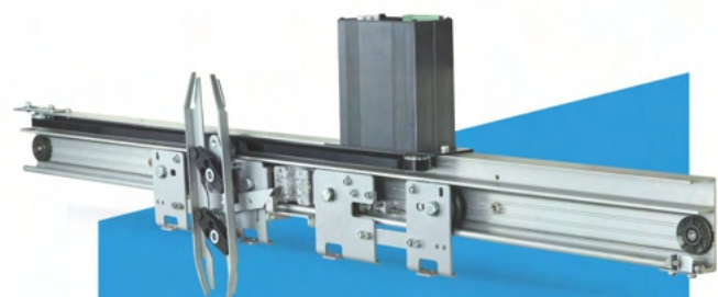
Center Opening Auto Door (Small Vision)
