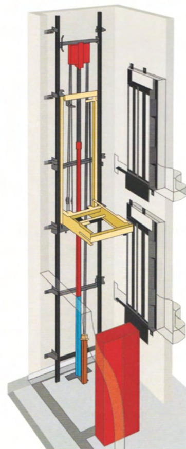
Hydraulic Elevator (Rope Type)
