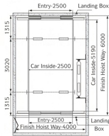
Hoistway Plan
